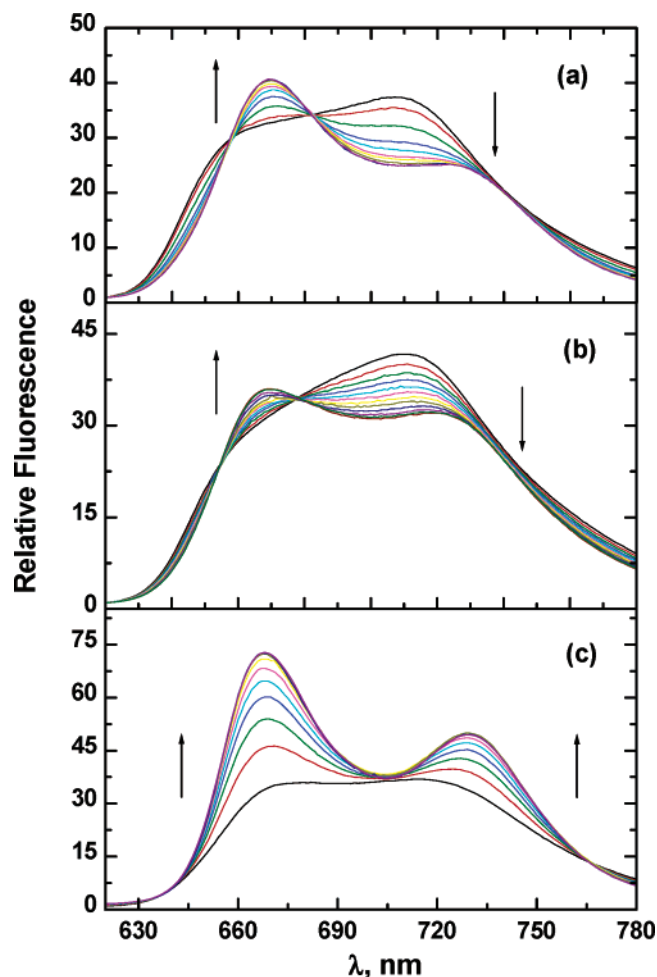
Figure 4. Fluorescence intensity spectra of TtOHPyP4 (panel a), TAlPyP4 (panel b), and TMetAlPyP4 (panel c) in the absence and presence of poly(rA)poly(rU) at 25 °C. The initial concentrations of the porphyrins were \sim 7 \mu\text{M} . The final RNA-to-ligand ratios were 9.3, 21.8, and 37.9 for TtOHPyP4, TAlPyP4, and TMetAlPyP4, respectively. The individual values of the final RNA-to-ligand ratio for each titration were selected to ensure saturation of the binding profiles.
