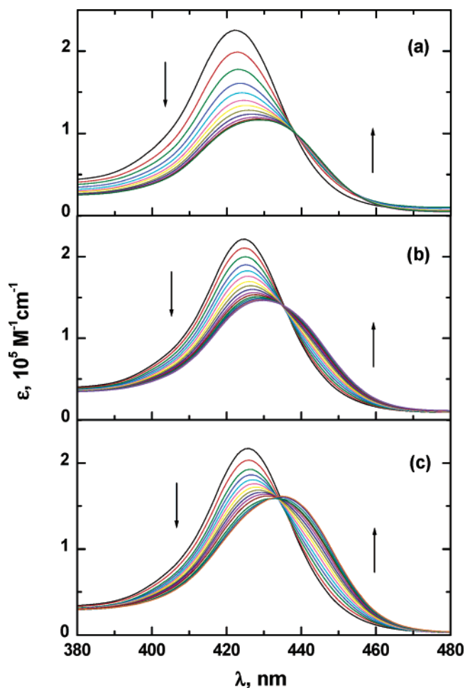
Figure 3. Visible absorption spectra of TtOHPyP4 (panel a), TAlPyP4 (panel b), and TMetAlPyP4 (panel c) in the absence and presence of poly(rI)poly(rC) at 25 °C. The initial concentrations of the porphyrins were \sim 5 \mu\text{M} . The final RNA-to-ligand ratios were 20.6, 60.9, and 65.2 for TtOHPyP4, TAlPyP4, and TMetAlPyP4, respectively. The individual values of the final RNA-to-ligand ratio for each titration were selected to ensure saturation of the binding profiles.
